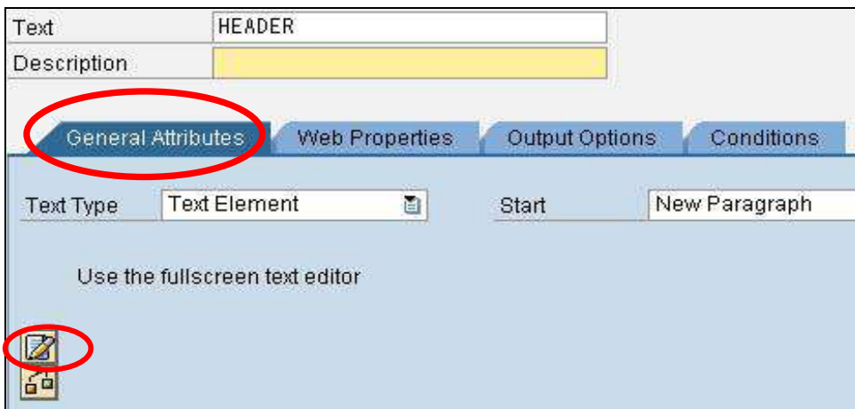
Figure 40 Adding Text
