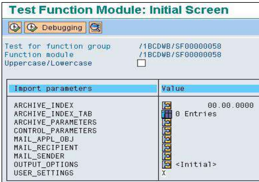
Figure 48 Printing Screen
