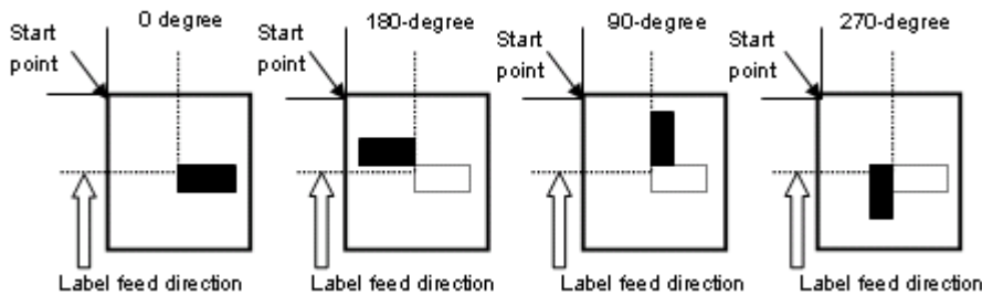
Figure 54 Rotation result
