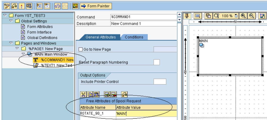
Figure 53 Text Rotation
