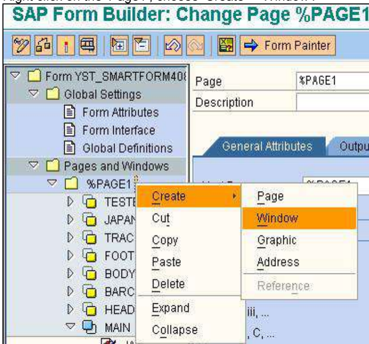
Figure 37 Creating Window
