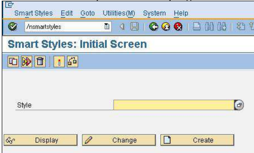
Figure 30 SmartStyles
